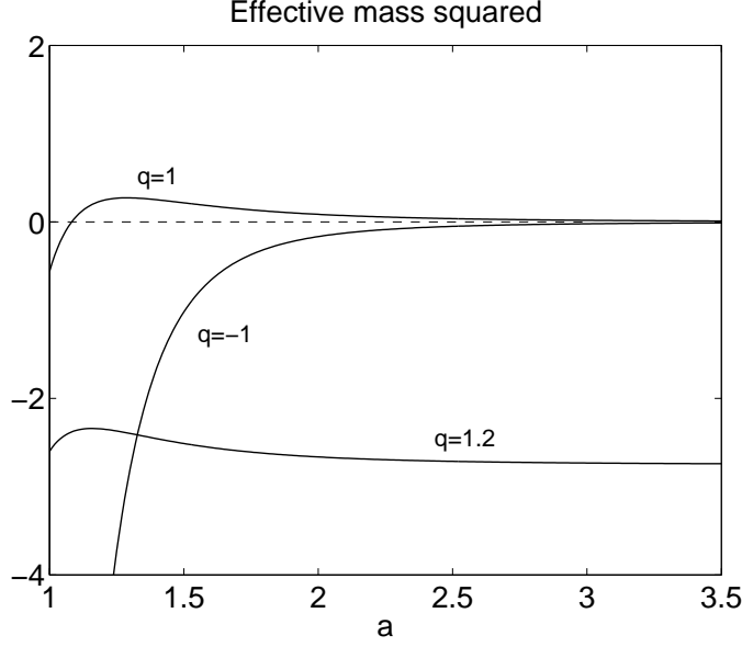
Figure 4: The dimensionless quantity M^2 \ell^2 as a function of a for E = 1, \ell = 1, r_H = 1 . Here, the effective mass squared is positive in a certain range only for the BPS-brane. Note that the negative M^2 \ell^2 region is not hidden behind the horizon.
