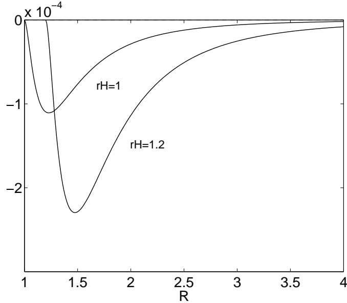
Figure 1: V_{\text{eff}}^t(E, q, R) for E = 0 , q = 1 , \ell = 4 and different values of r_H . For R \rightarrow \infty the potential goes to zero according to our normalization. When r_H = 0 , the potential is exactly flat.
