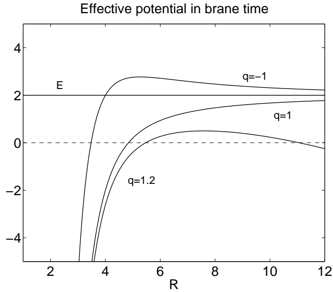
Figure 3: V_{\text{eff}}^\tau(E, q, R) for the same parameters as in Fig.2. A BPS brane has zero kinetic energy at infinity corresponding to a vanishing cosmological constant on the brane. Otherwise, the cosmological constant is \propto q^2 - 1 . A BPS anti-brane is allowed to move only in a restricted range of R : after having reached a maximal scale factor, the universe starts contracting. Any inwardly moving brane falls into the black hole in a finite \tau .
