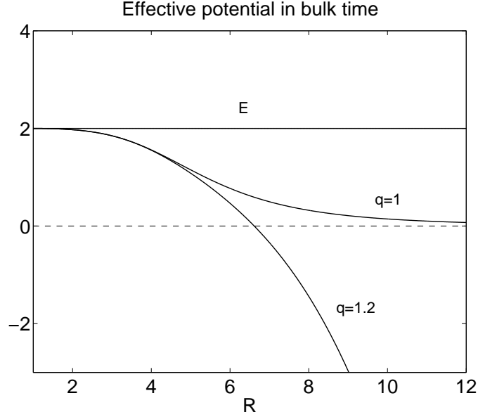
Figure 2: V_{\text{eff}}^t(E, q, R) for E = 2 , r_H = 1 , \ell = 4 . For a BPS-brane ( q = 1 ), V_{\text{eff}}^t \rightarrow 0 as R \rightarrow \infty according to our normalization. This should be contrasted with a non-BPS brane e.g. with q = 1.2 . Note that V_{\text{eff}}^t(E, q, R = r_H) = E . Any inwardly moving (contracting) brane takes an infinite amount of t -time to reach the horizon.
