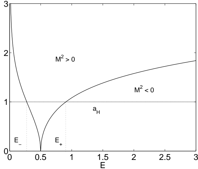
Figure 5: The curve represents a_c , the zero of M^2(\tau) , as a function of the energy E as given in Eq. 3.30. Below the curve the effective mass squared is negative, above it is positive. For E < E_- and E > E_+ the M^2(\tau) becomes negative already outside the horizon, whereas for energies within the interval E_-, E_+ the M^2(\tau) < 0 region is hidden within the horizon. The parameters chosen are q = 1, r_H = 1 and \ell = 1 .
